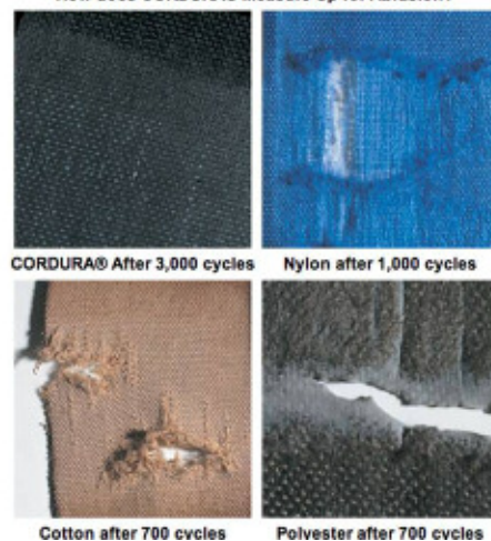
How does CORDURA® Measure Up for Abrasion?
